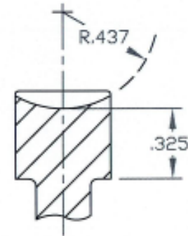
SLOTTING DETAIL
